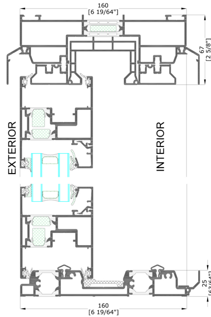
DETAIL 3
